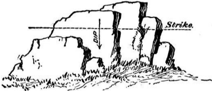
Outcrop of Rock, showing Dip and Strike.
